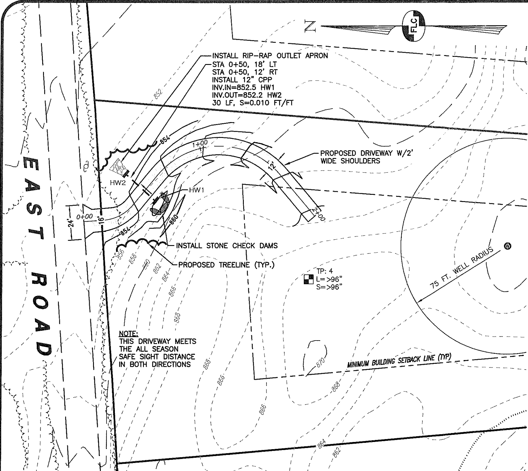
DRIVEWAY PLAN
