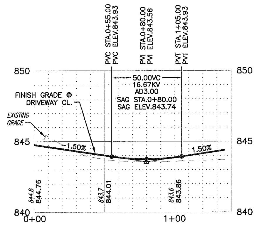
DRIVEWAY PROFILE
