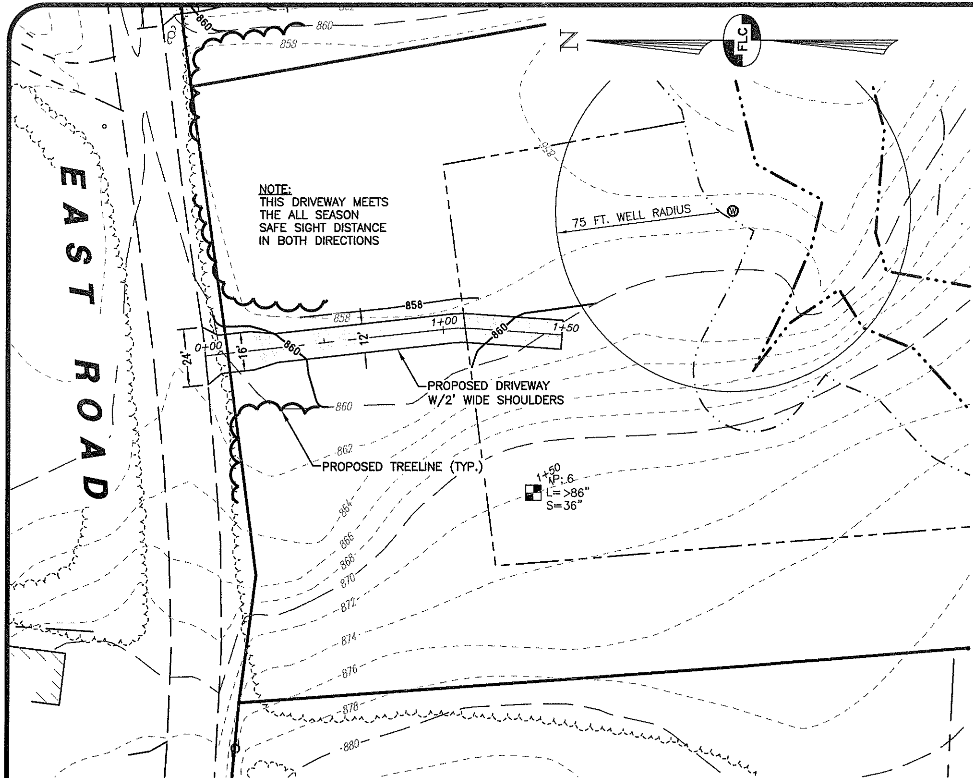
DRIVEWAY PLAN
