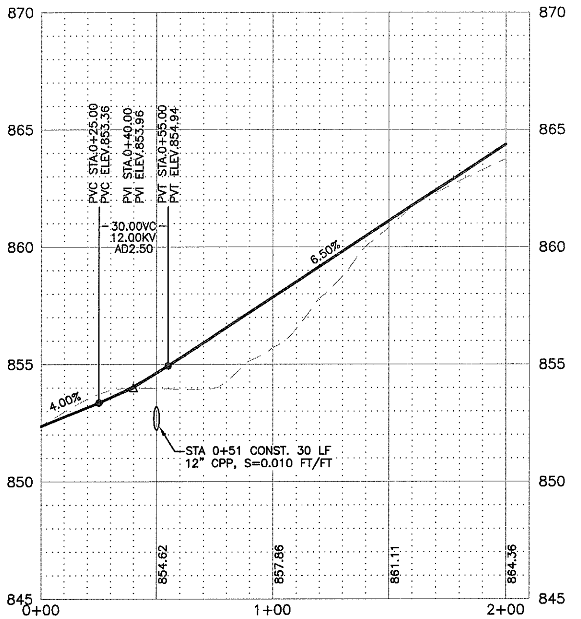
DRIVEWAY PROFILE
