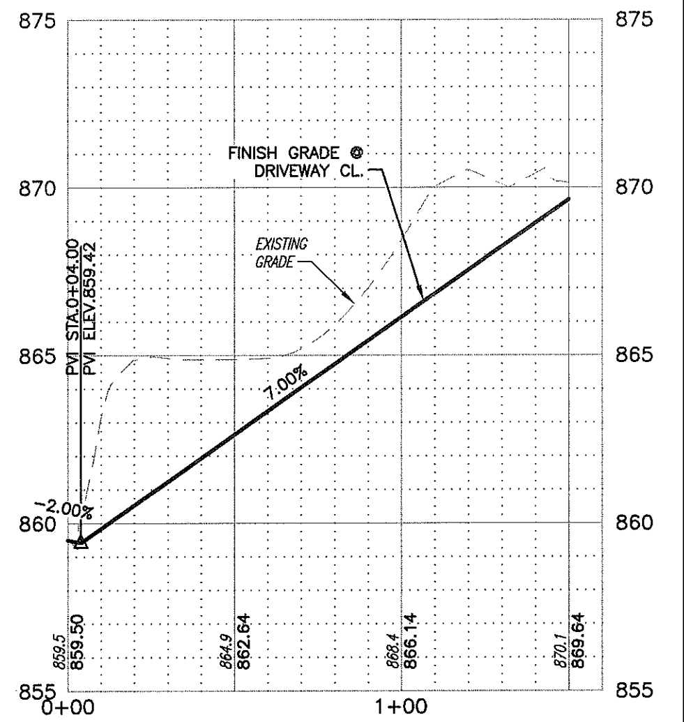
DRIVEWAY PROFILE
