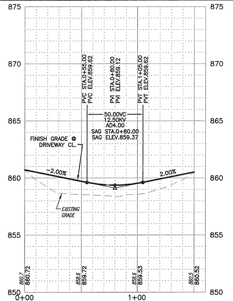
DRIVEWAY PROFILE
