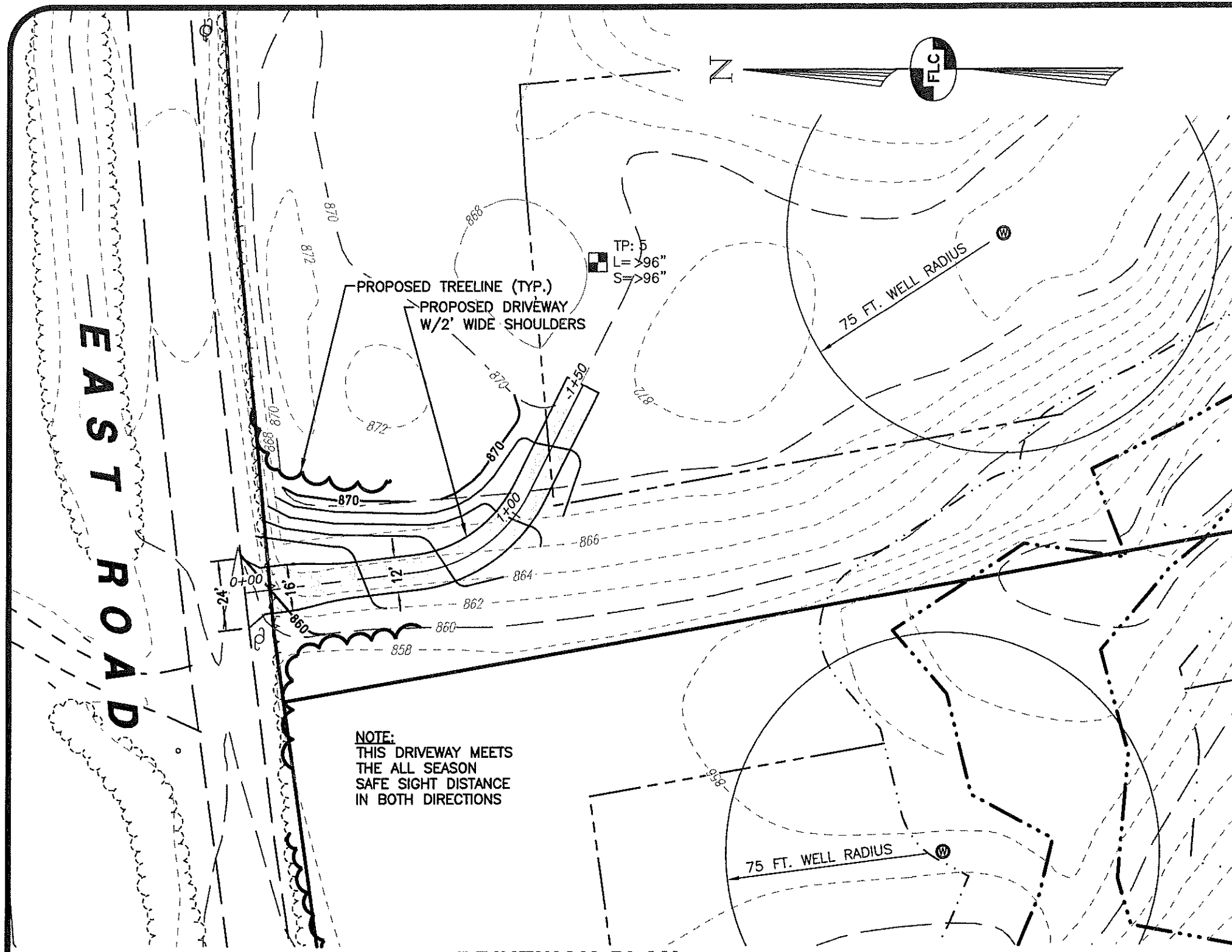
DRIVEWAY PLAN
